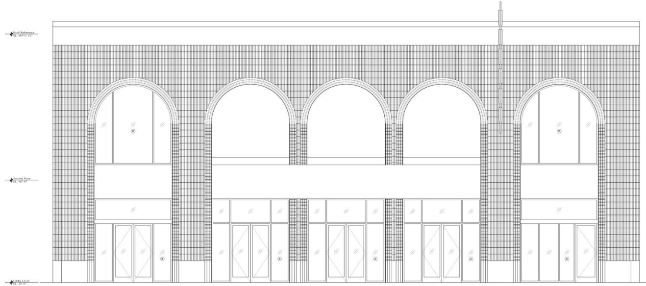
43 South Exterior Elevation SCALE: 3/8" = 1'-0"
